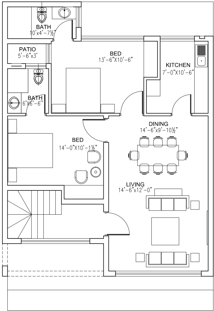
FIRST FLOOR
